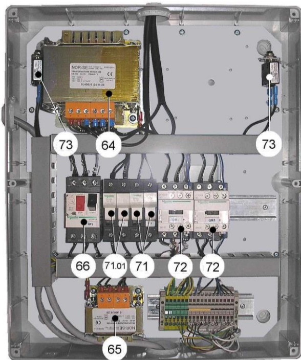
electrical system with heat protection on sealing bars
